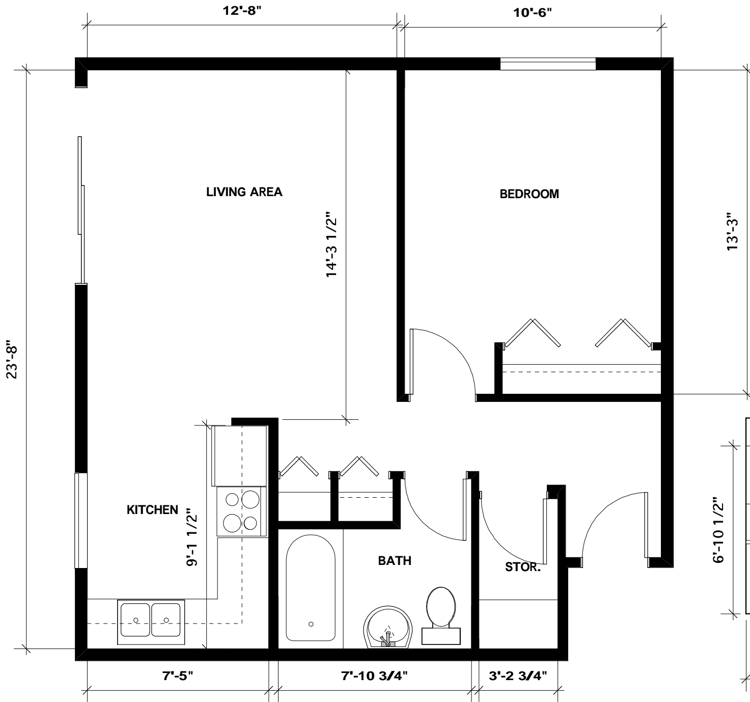
1 TOTAL AREA 575.5 SQ. FT. SCALE 1/4"=1'-0"
