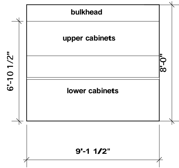
2 KITCHEN ELEVATION Scale: 1/4" = 1'-0"
