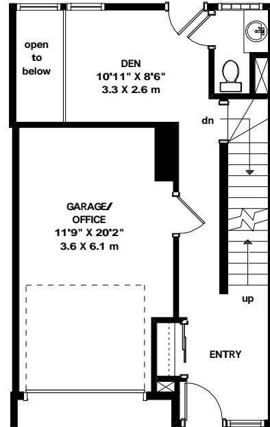
MAIN FLOOR 348.9 SQ. FT. 32.4 m2
