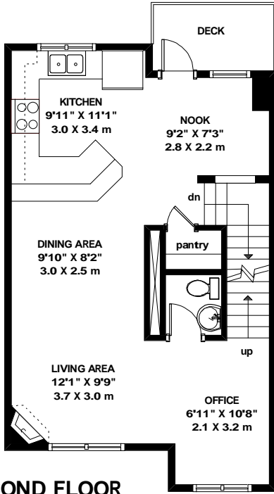
SECOND FLOOR 610 SQ. FT. 56.7 m2
